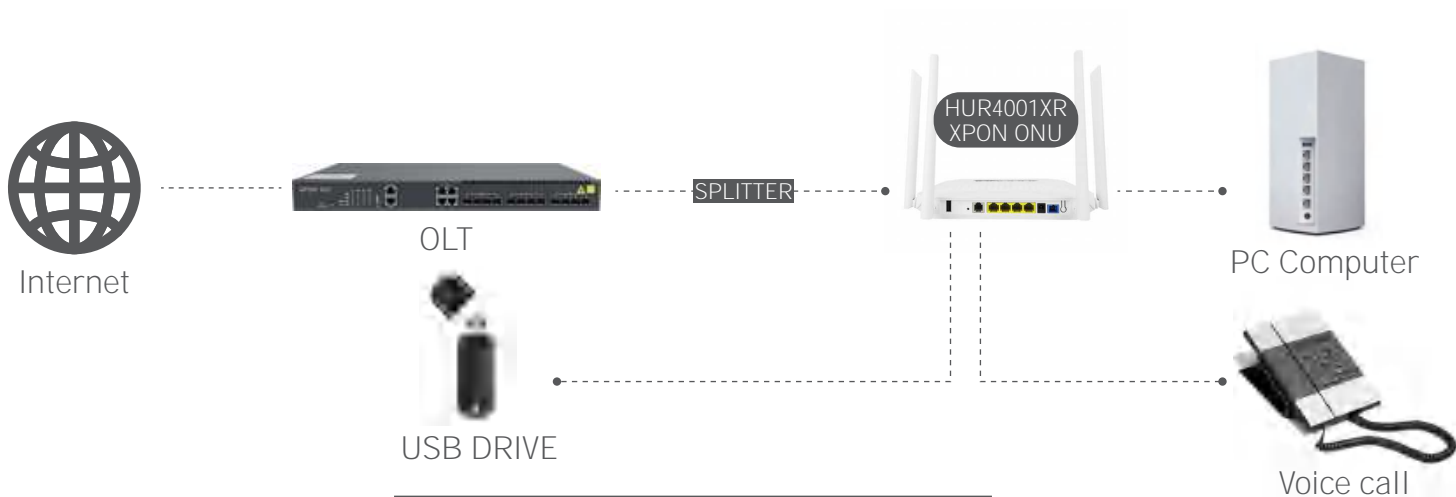
Figure: HUR4001XR Application Diagram
