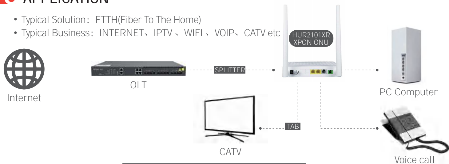
Figure: HUR2101XR Application Diagram
